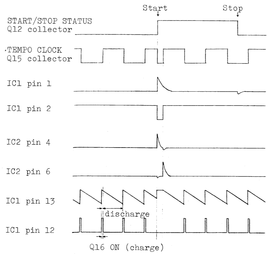
FIGURE 9 TEMPO CLOCK TIMING DIAGRAM
